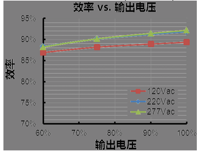
EUP-096S150ST (Io=1500mA)
